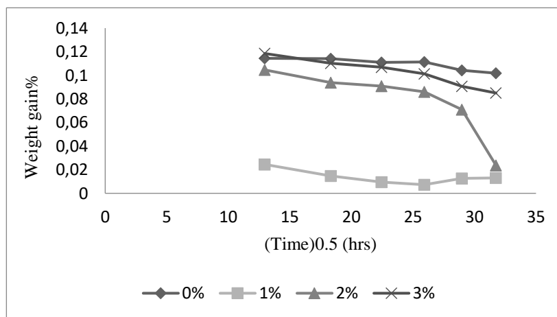
Fig. 5. Weight gain % vs square root time of immersion of all samples
